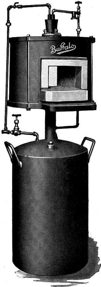
Buffalo No. 3 Oil-Burning Rivet Forge.
