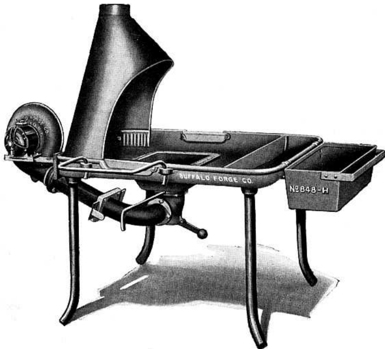
Buffalo No. 848-H Forge with Electric Blower
