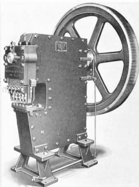
No. 45 Rapid Acting Punch with multiple head.
