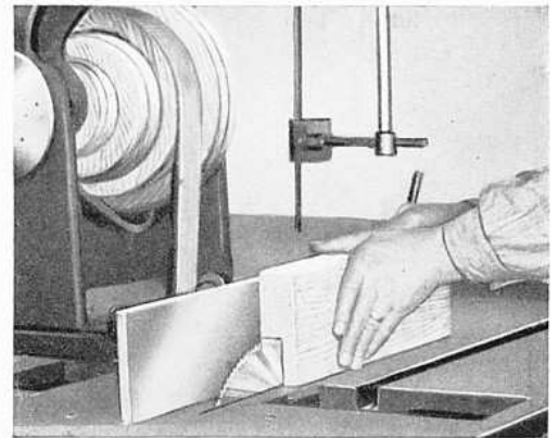
Mortising With Circular Saw
