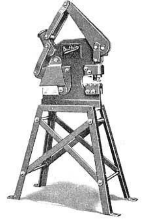
No. 2B Punch and Shear with compounded leverage.
