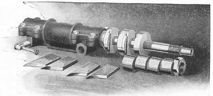
Mandrel for Jointer, Shaper and Circular Saw
