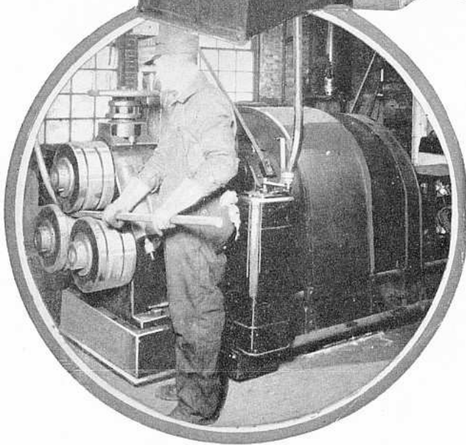
The material being handled in this Buffalo Vertical Bending Roll is 4" x 5" structural steel angle, ½" thick and 12' 5" long.
