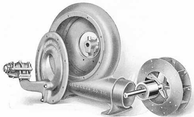
Parts of Steel Pressure Blower
