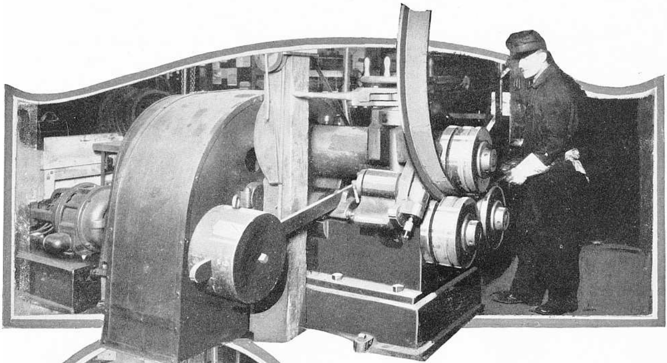
The material being handled in this Buffalo Vertical Bending Roll is 4" x 5" structural steel angle, ½" thick and 12' 5" long.
