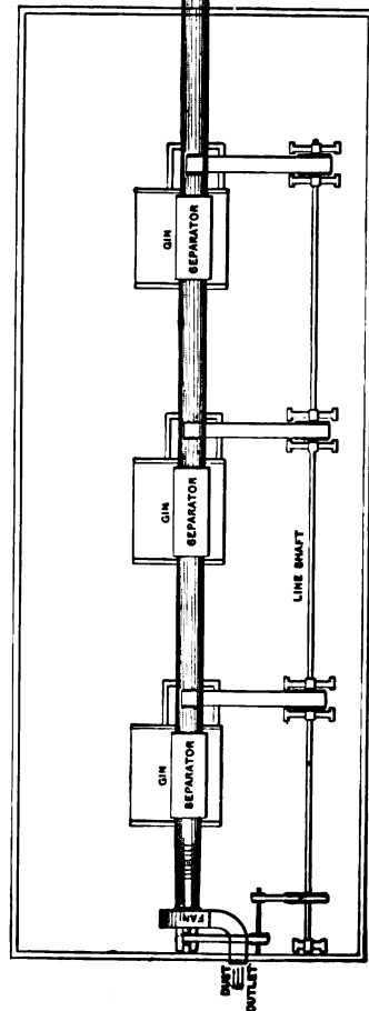
PLAN OF GIN-HOUSE
