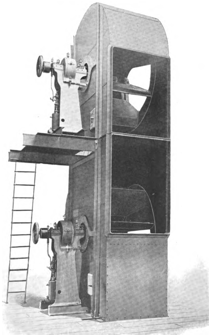
Single Engines, Left Hand Fans, Bottom and Top Horizontal Discharge, Overhung Wheels and Water-cooling Bearings.
