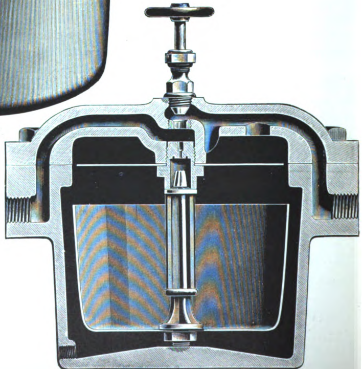
Sectional View.
