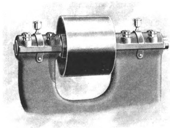
Outside View of Oil Ring Bearing.
