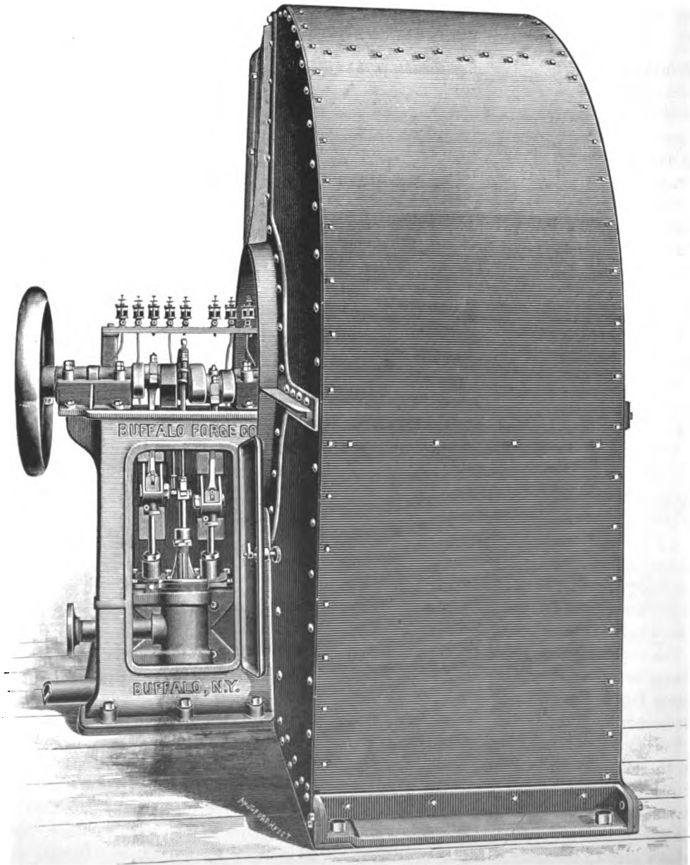
Engine Cylinders Beneath the Shaft. Fan Right Hand Top Horizontal Discharge, with Overhung Wheel. For Mechanical Draft, Ship Ventilation, Etc.
