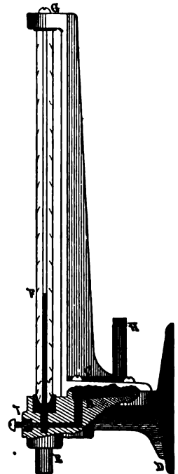
Pressure Gauge, Side Section.
