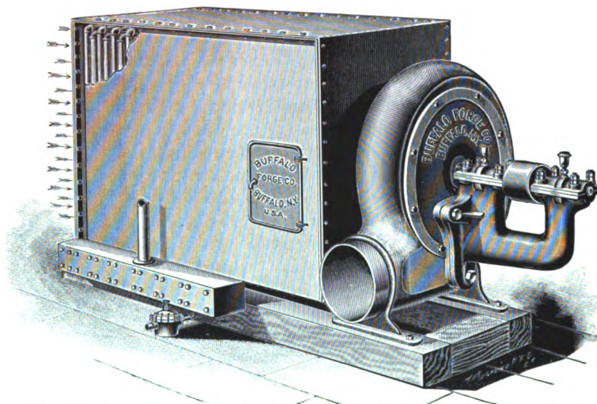
Fig. 1. Right Hand Bottom Horizontal Discharge, "B" Volume Exhaust Pulley Fan, Drawing Through Heater.
