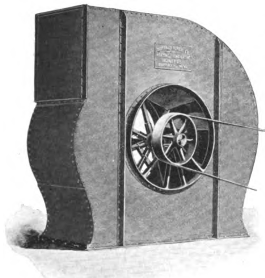
Right Hand Top Horizontal Discharge Blower.
