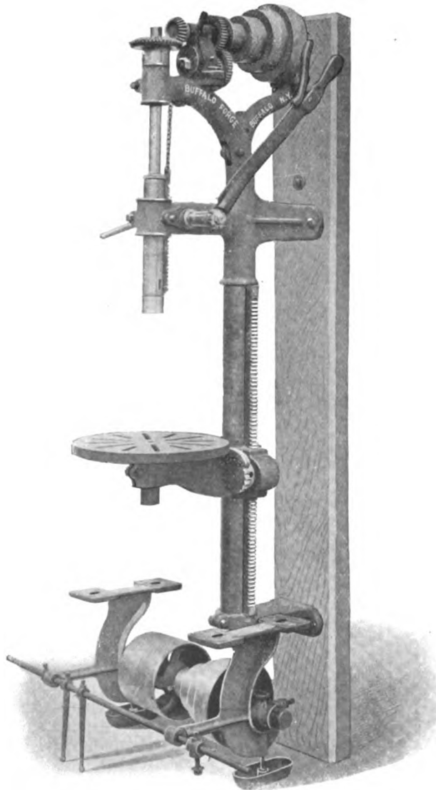
No. 88 Power Drill, with Back Gear.
