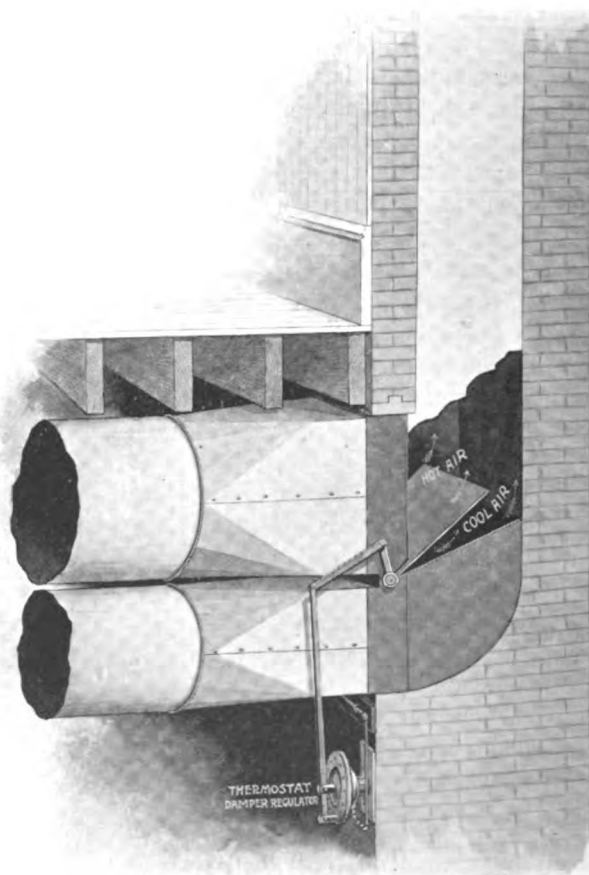
Buffalo Air-mixing Damper Controlled by a Thermostat.
