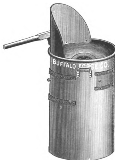
No. 10 Hand Forge.
