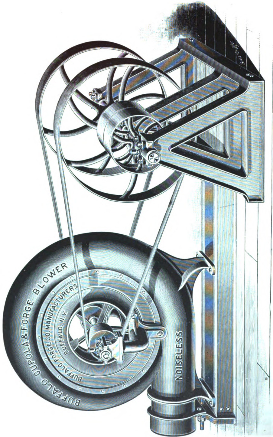
Right Hand Apparatus, Tight and Loose Countershaft Pulleys, Blower Bottom Horizontal Discharge. Also Built Left Hand.
