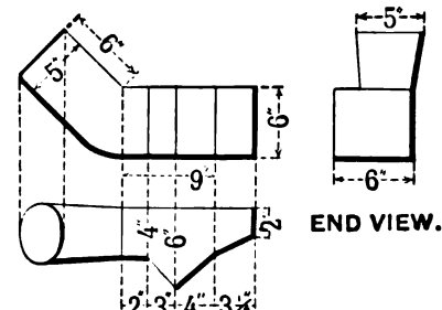
SIDE VIEW AND PLAN.
